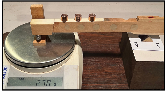
Figure 1: Front weight of 27g mocked up with 13.2g soft copper key weights using home made jig with wedge and playing cards for leveling.
