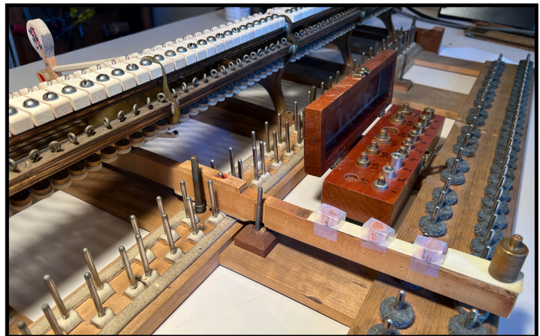
Figure 3: Checking for a 38 test balance weight
